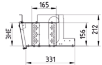
Sectional drawing of cable trough
